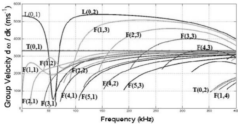
Fig 1. Group velocity dispersion curves for the steel pipe (Outer diameter: 34 mm, wall thickness: 5.5 mm.). [Ref:B. Zaghari etal, Proc. 19th Intern. Conf. on Automation & Computing, Brunel University, London, UK, 13-14 September 2013]
